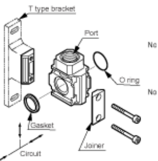
D101 Distributor Block
